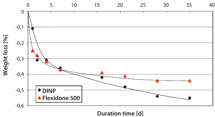
Weight Loss at 80°C, at the same Shore A
